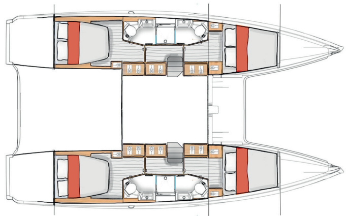
VERSION 4 CABINES
