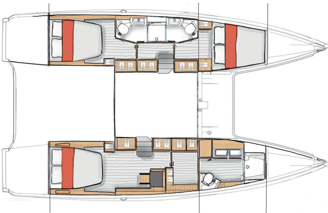
VERSION 3 CABINES
